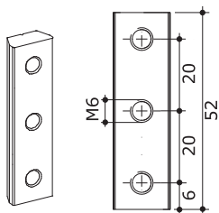
Nutenstein grooved guide NUT.15-523M6-00
