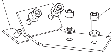
Konsole links bracket left
