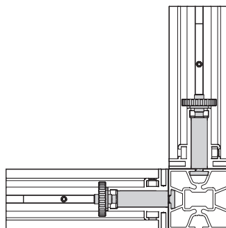
Rahmen / GAMMA-52 frame / GAMMA-52
