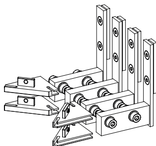
Verbinder-Sets connector sets
