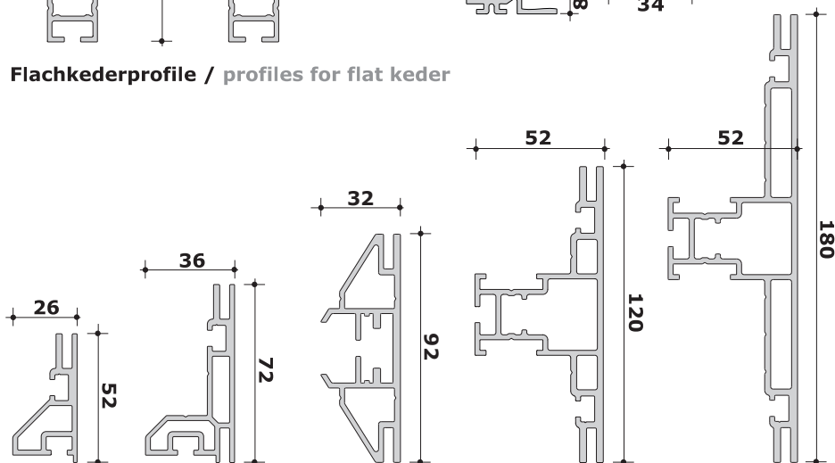
LED-Flachkederprofile / LED profiles for flat keder
